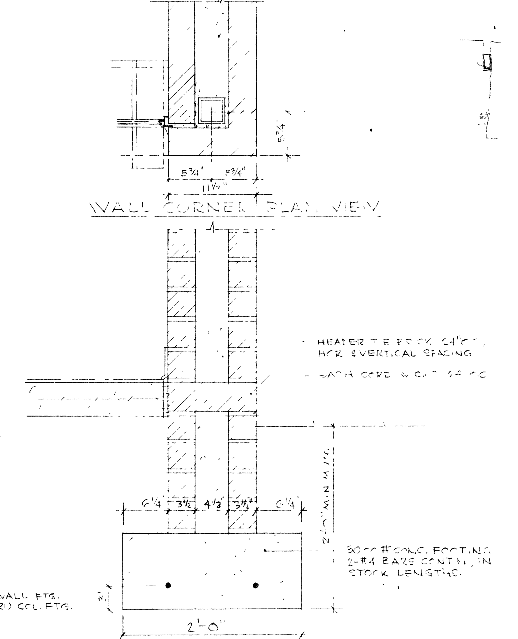
EXTERIOR WALL COL-BEAM DETAIL TYPICAL END WALL SECTION
