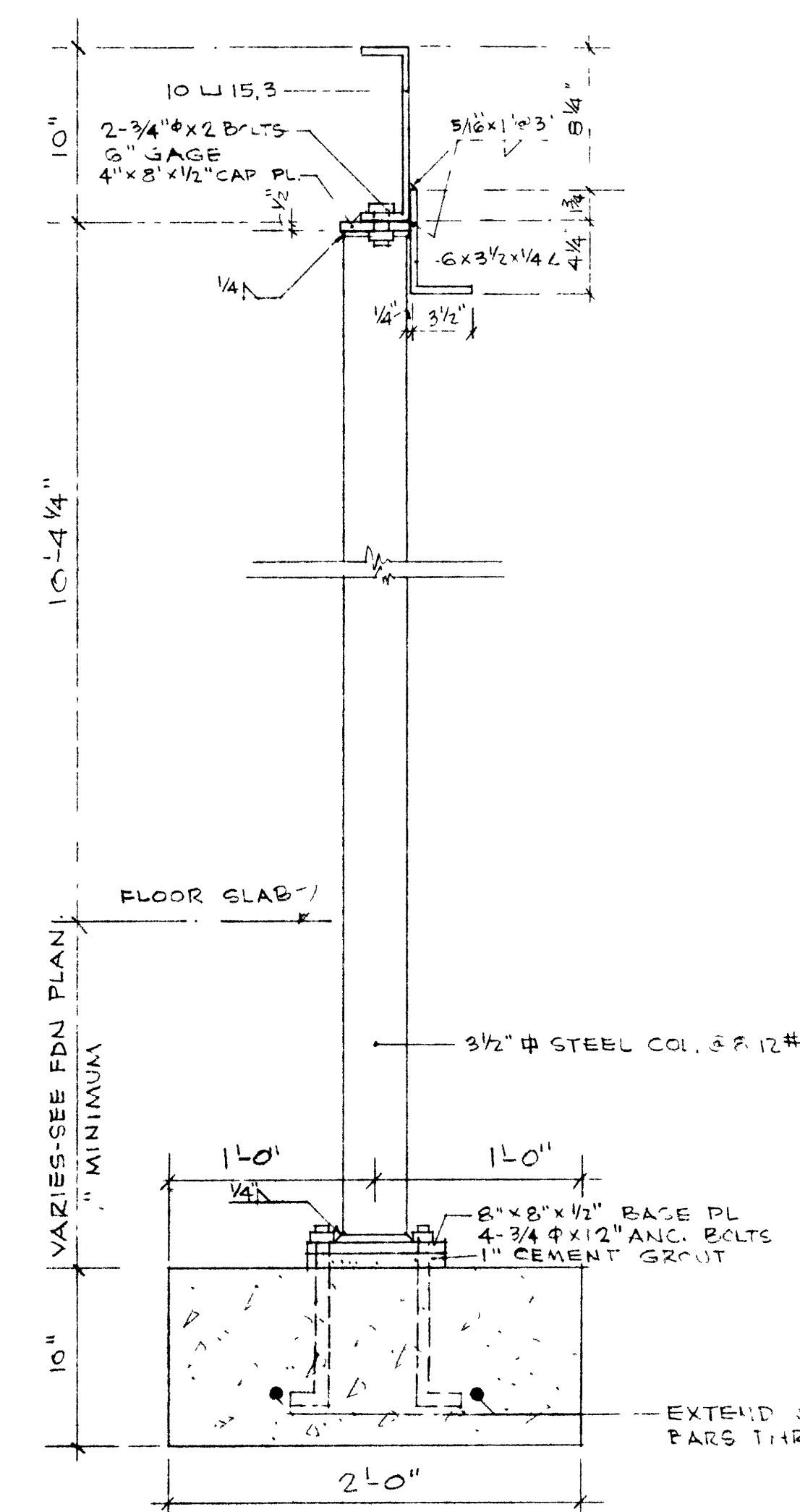
EXTERIOR WALL COL-BEAM DETAIL TYPICAL END WALL SECTION
