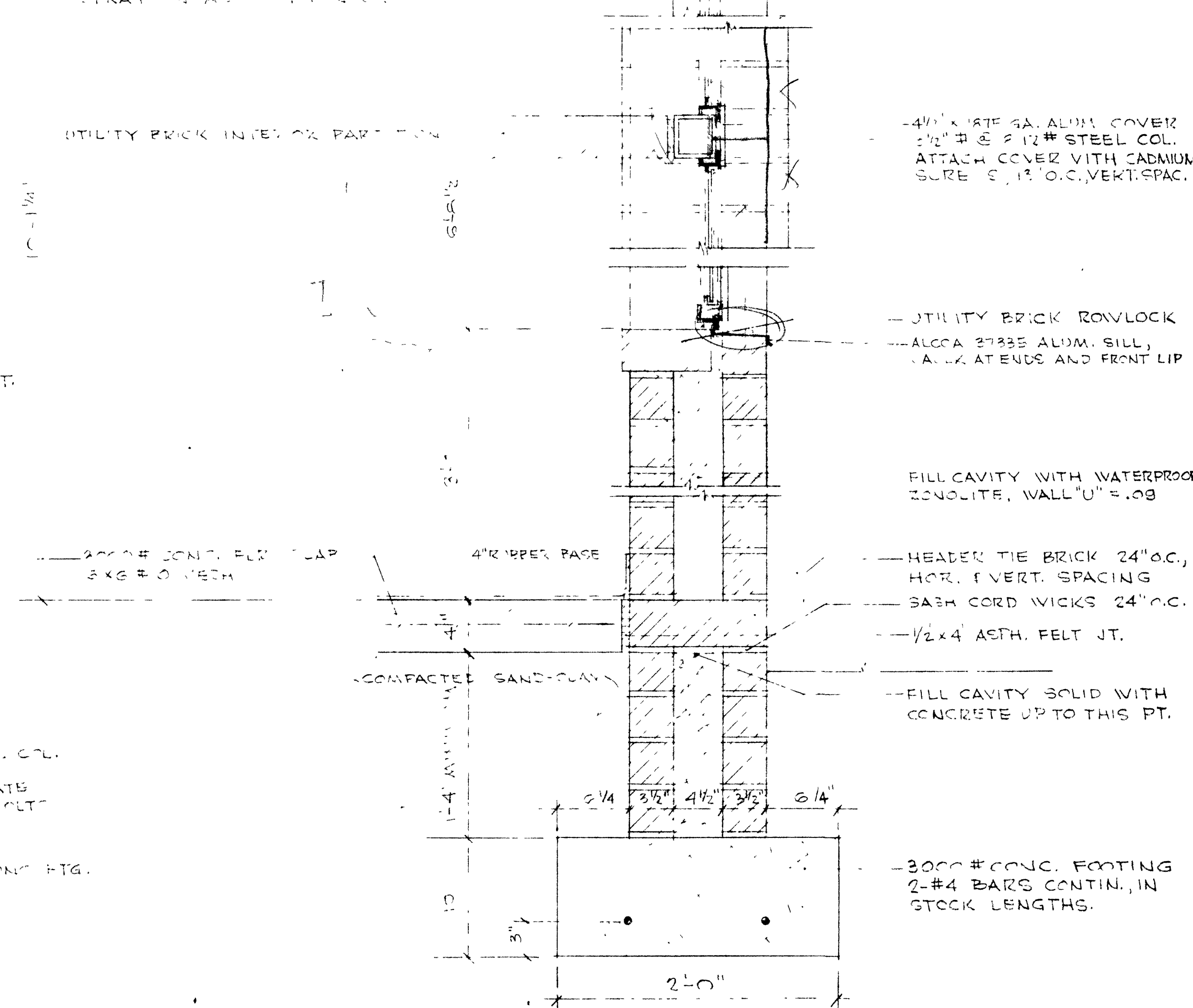
TYPICAL EXTERIOR SIDEWALL SECTION 1/2\"/>
