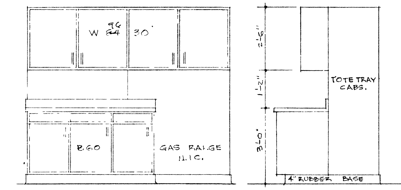
HOME EC. ISLAND CAB.
