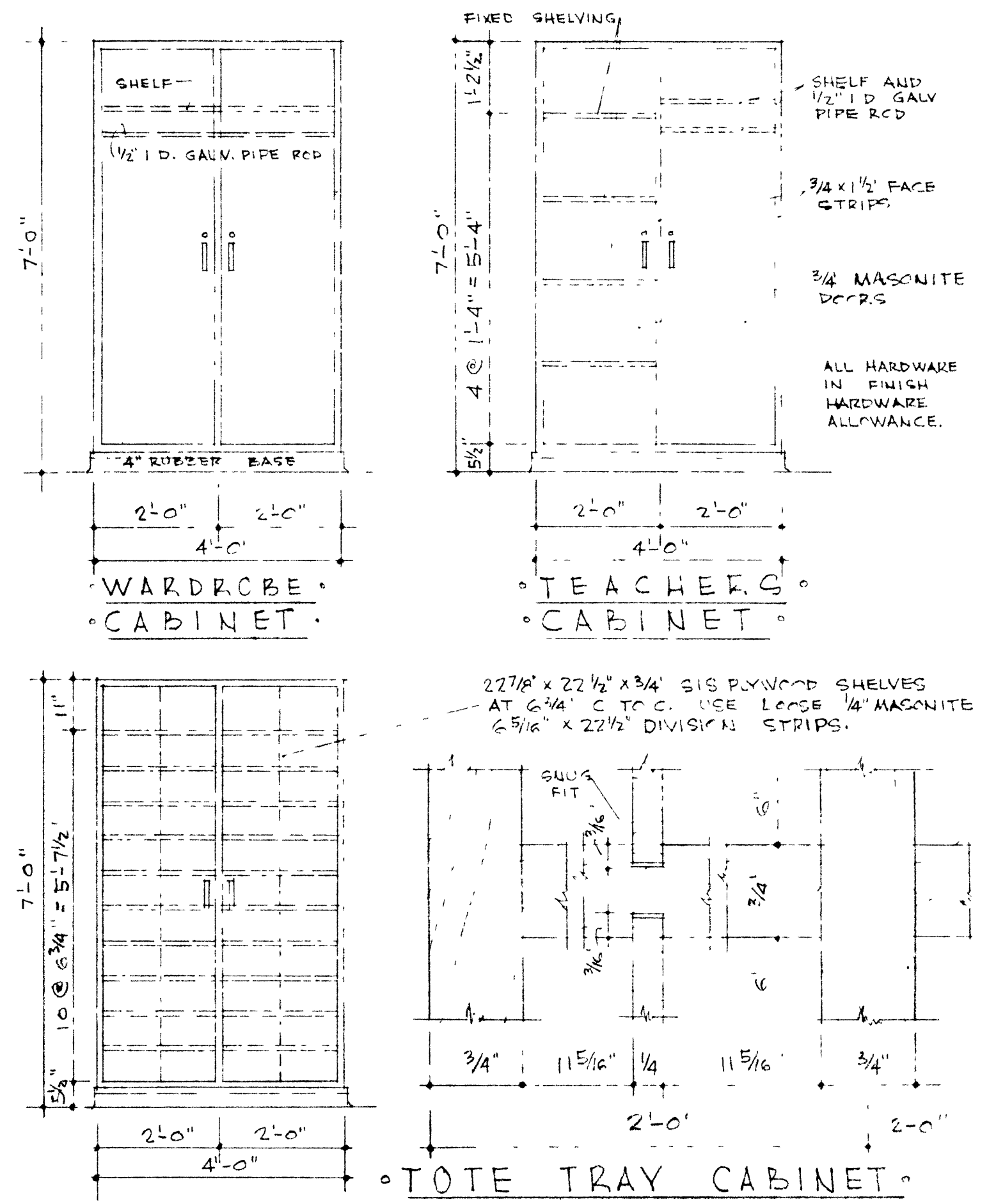
TYPICAL DETAILS FOR CABINETS
