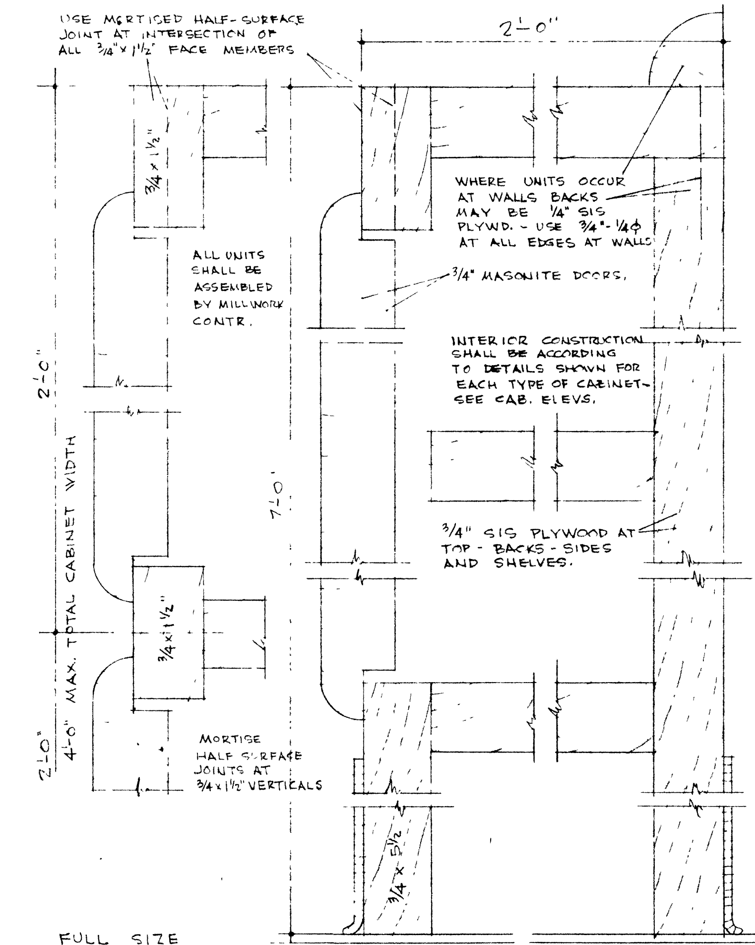
FULL SIZE THESE DETAILS TYPICAL FOR WARDROBE, IRONING BD, TOTE TRAY, STORAGE, AND TEACHERS CABINETS.
