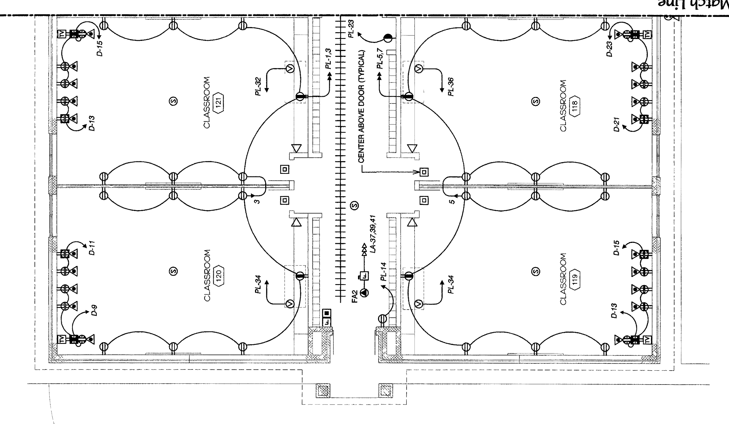
1 FLOOR PLAN "A" - POWER/COMMUNICATIONS 1/8" = 1'-0"
