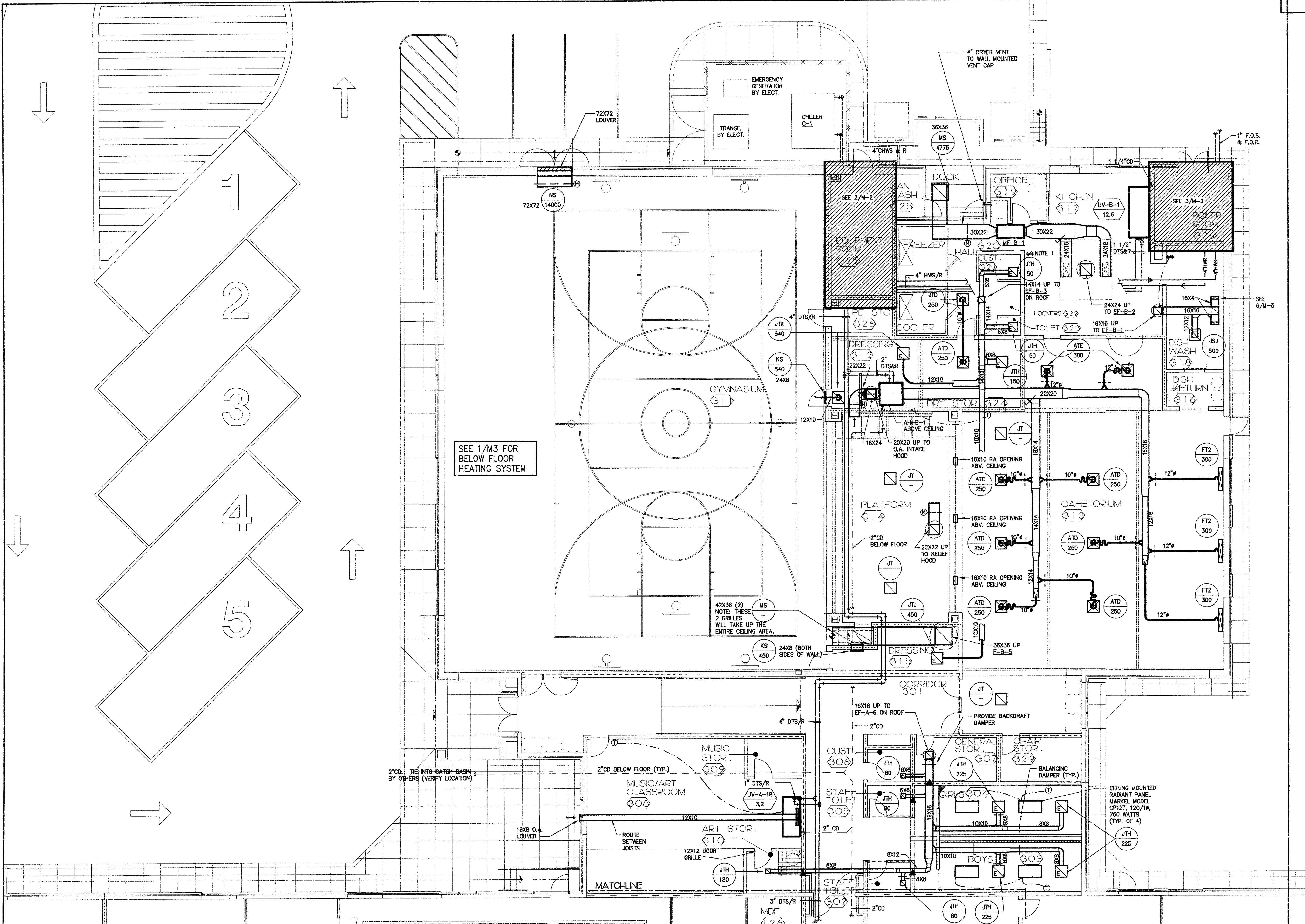
1 FLOOR PLAN "B" M-2 1/8"=1'-0"
