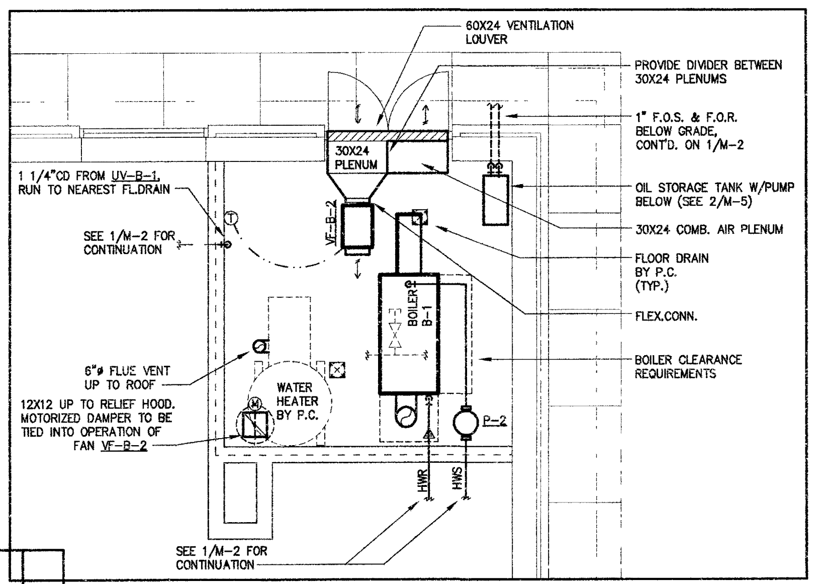
3 BOILER ROOM 326 M-2 1/4"=1'-0"
