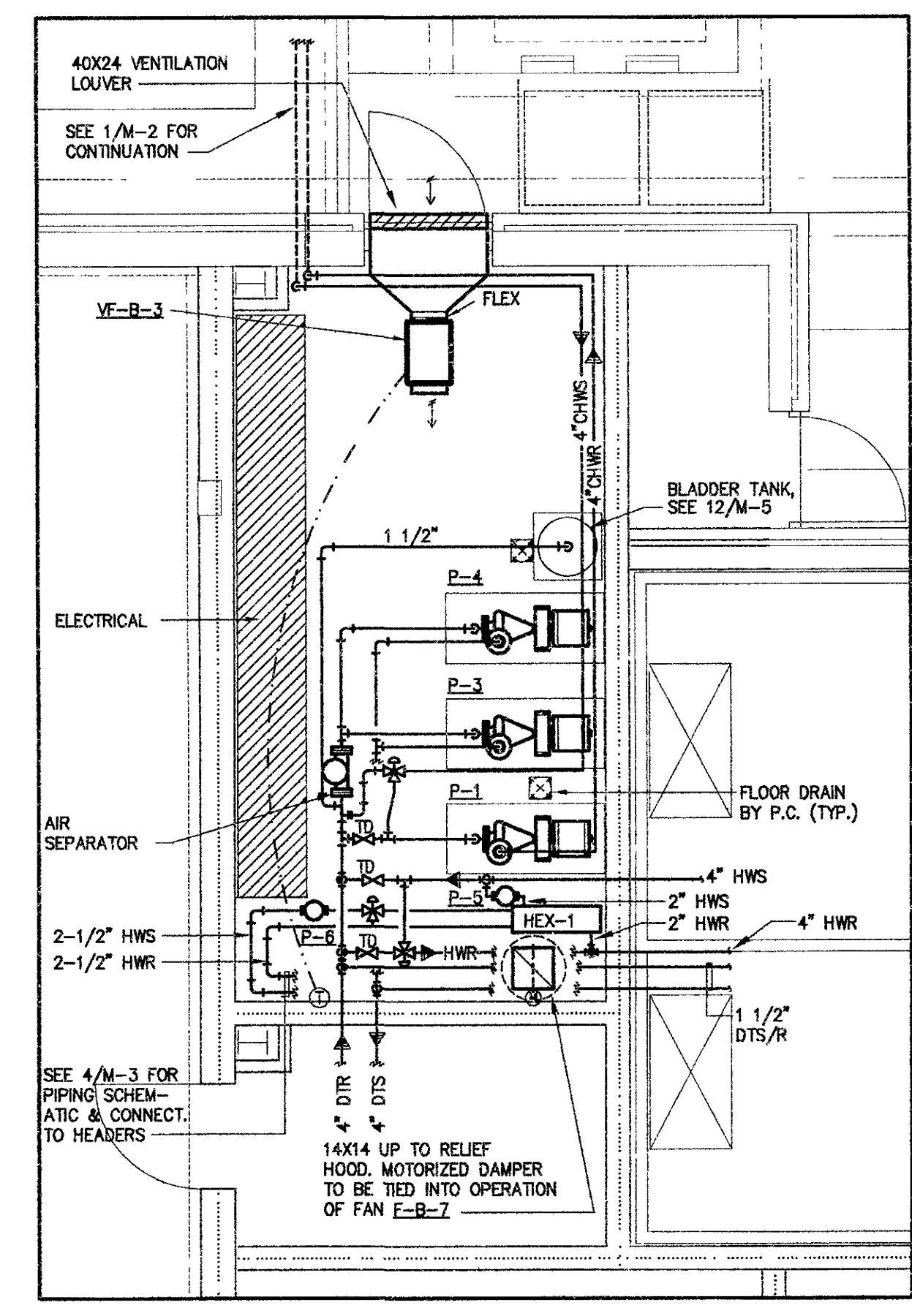
2 EQUIPMENT ROOM 325 M-2 1/4"=1'-0"
