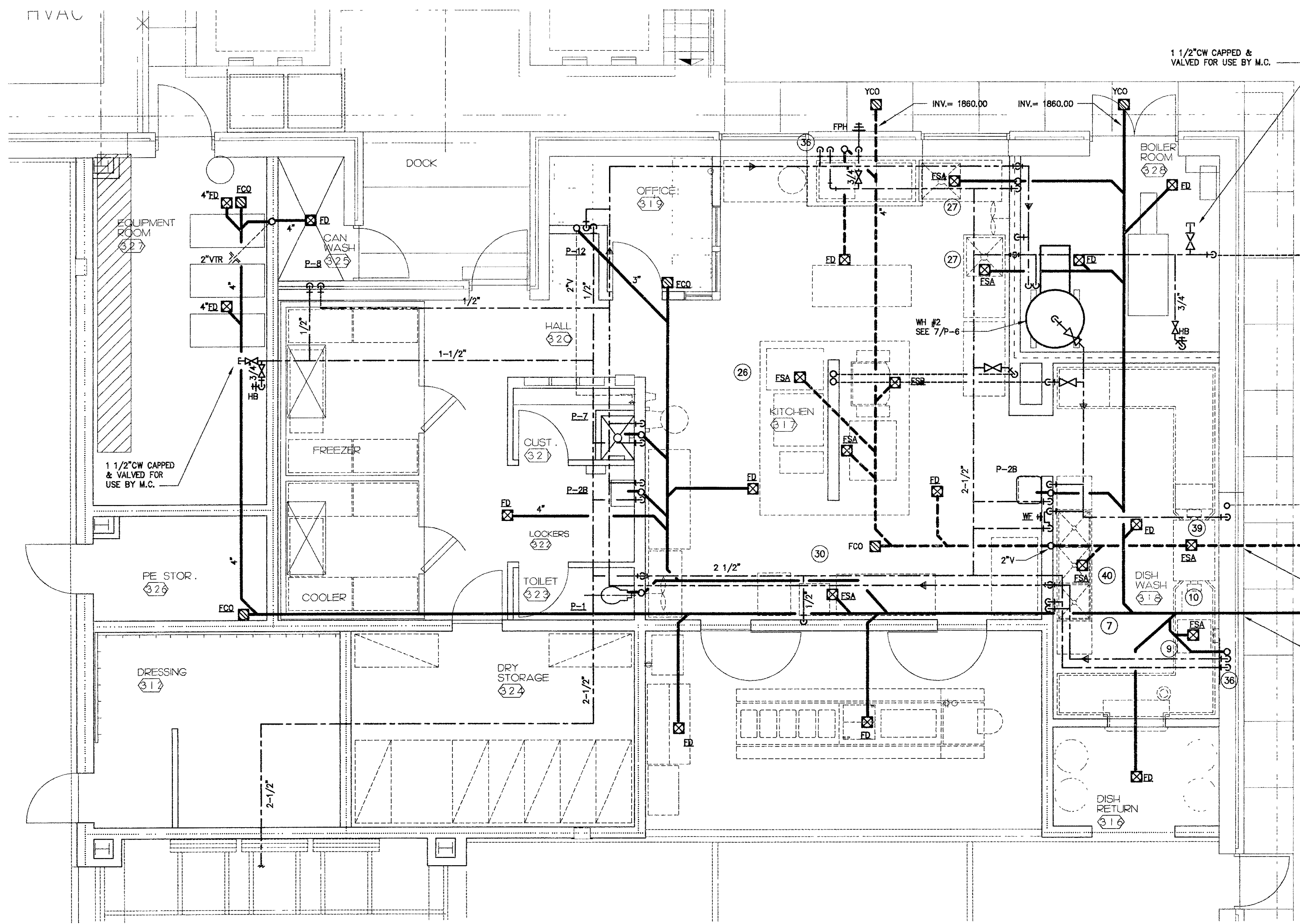
1 FLOOR PLAN 'B' P-4 1/4"=1'-0" FFE = 1863'
