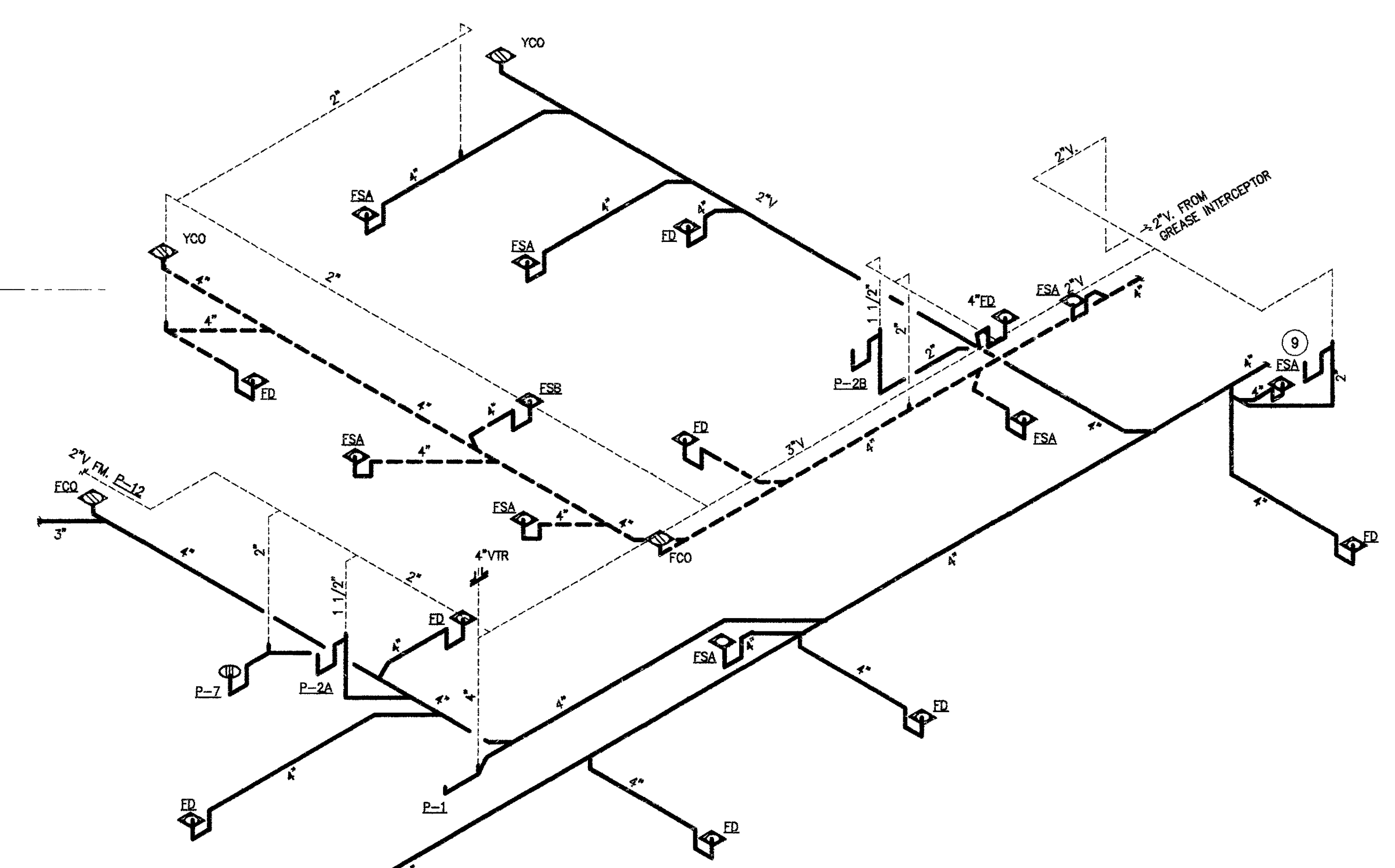
3 WASTE PIPING SCHEMATIC P-4 NTS
