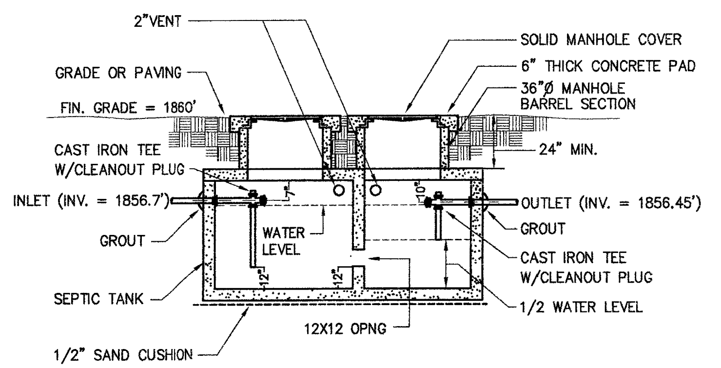
4 GREASE INTERCEPTOR DETAIL P-4 NTS (1500 GAL. PRECAST)
